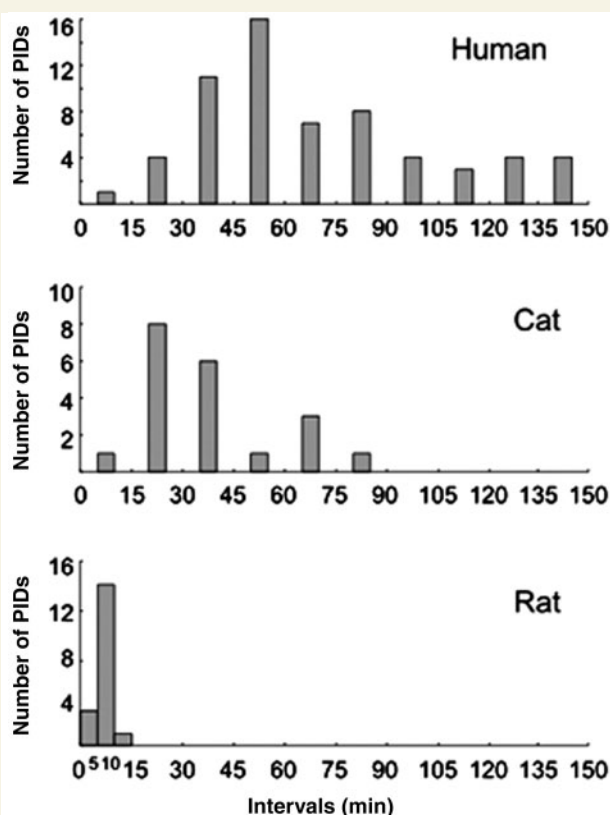
Figure 6 Inter-species comparison of CSD periodicity. Time interval histograms are shown between recurrent cyclic CBF IND waves after dMCAO in rats ( n=6 ), circumferential CBF IND waves after proximal MCA occlusion in cats ( n=7 ) and spreading depolarizations in human malignant hemispheric stroke appearing in clusters of CSD ( n=7 ). Please note that intervals propagating unidirectionally were analysed in cats and human patients. Distributions reveal (i) intervals to be shorter in rats than in cats and humans and (ii) that in humans, intervals are distributed more widely than in cats and rats.
