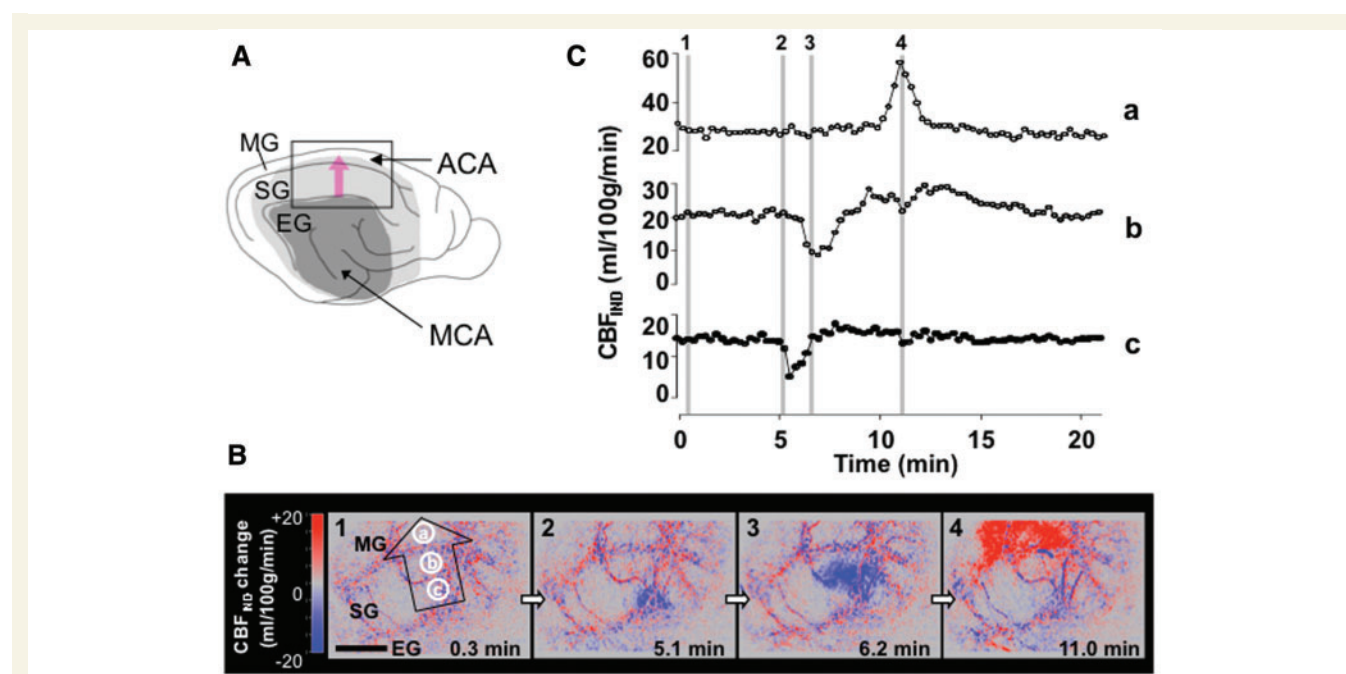
Figure 3 Radial CBF IND wave propagation in the ischaemic boundary zone after cat MCA occlusion (see also Supplementary Video 2). (A) Diagram of the lateral aspect of the cat brain with schematic representation of ischaemic core (dark grey) and border zone (light grey) after MCA occlusion. Arrows indicate territories of MCA and anterior cerebral artery (ACA), pink arrow indicates radial direction of CBF IND wave propagation. (B) Sequential images (1–4) of radial CBF IND wave propagating from inner ischaemic boundary zone (suprasylvian gyrus; SG) to periphery (marginal gyrus; MG). Colour coded CBF IND change indicates hypoperfusion appearance in the suprasylvian gyrus near the ischaemic core in blue, hyperaemic appearance in the MG in red as the wave travels into the ischaemic periphery. Time in images indicates time from onset of CBF IND wave and corresponds to time scale in Fig. 4C. Regions of interest a, b, c in first image served for time course analysis (Fig. 4C). (C) Time course of CBF IND in regions of interest a, b and c, showing the transition from hypo- to hyperaemic appearance as the wave propagates from inner to outer boundary zone of the ischaemic focus. EG = ectosylvian gyrus.
